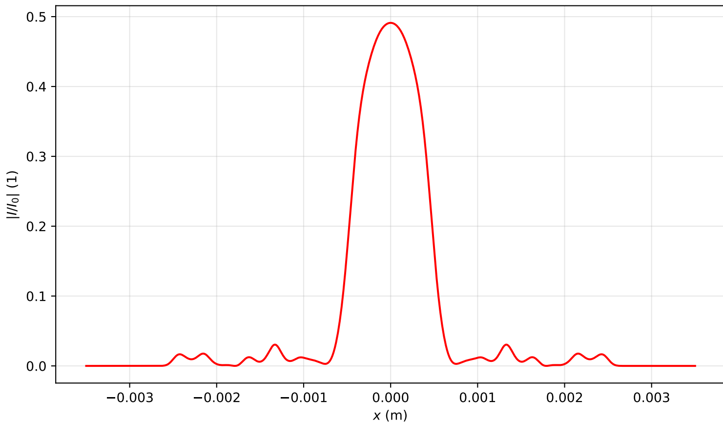
Intensity profile I(x, y = 0, z = 2.866)/I_0 , P_{in}=3.5P_{cr} , artificial time
